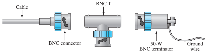
Figure 7.8 BNC connectors
